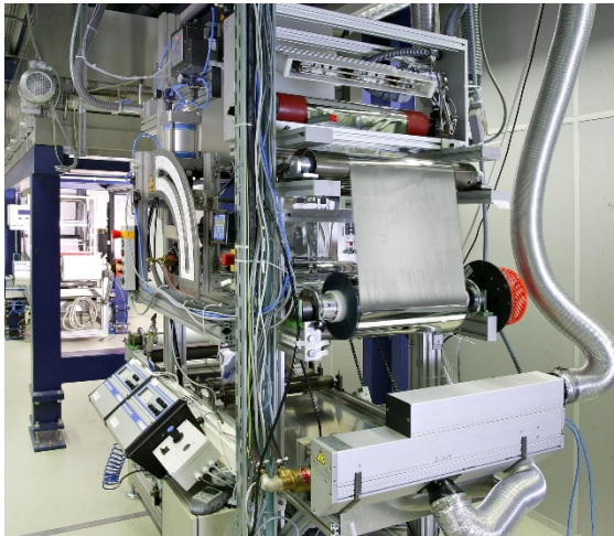
Fig. 2: In the coating process, the paper is guided over rolls and provided with the “BioActive Materials”. These are supplied in the form of an aqueous dispersion.
