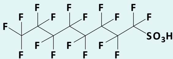
perfluorinated surfactants / industrial chemicals
