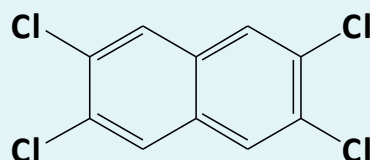
polychlorinated aromatics / flame retardants
